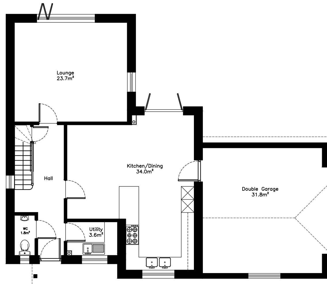
ground floor plan as proposed floor area = 77.6m 2 excluding garage
