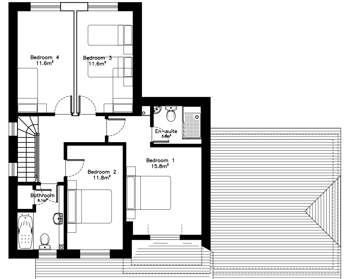
first floor plan as proposed floor area = 73.1m 2
